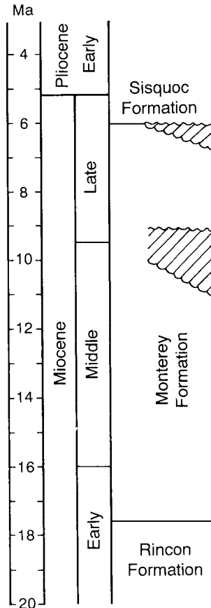
Figure 15. Conventional timescale for the Monterey Formation of California (after Barron). 18 In some places there is an erosion break within the Monterey Formation at the Middle-Late Miocene transition.
