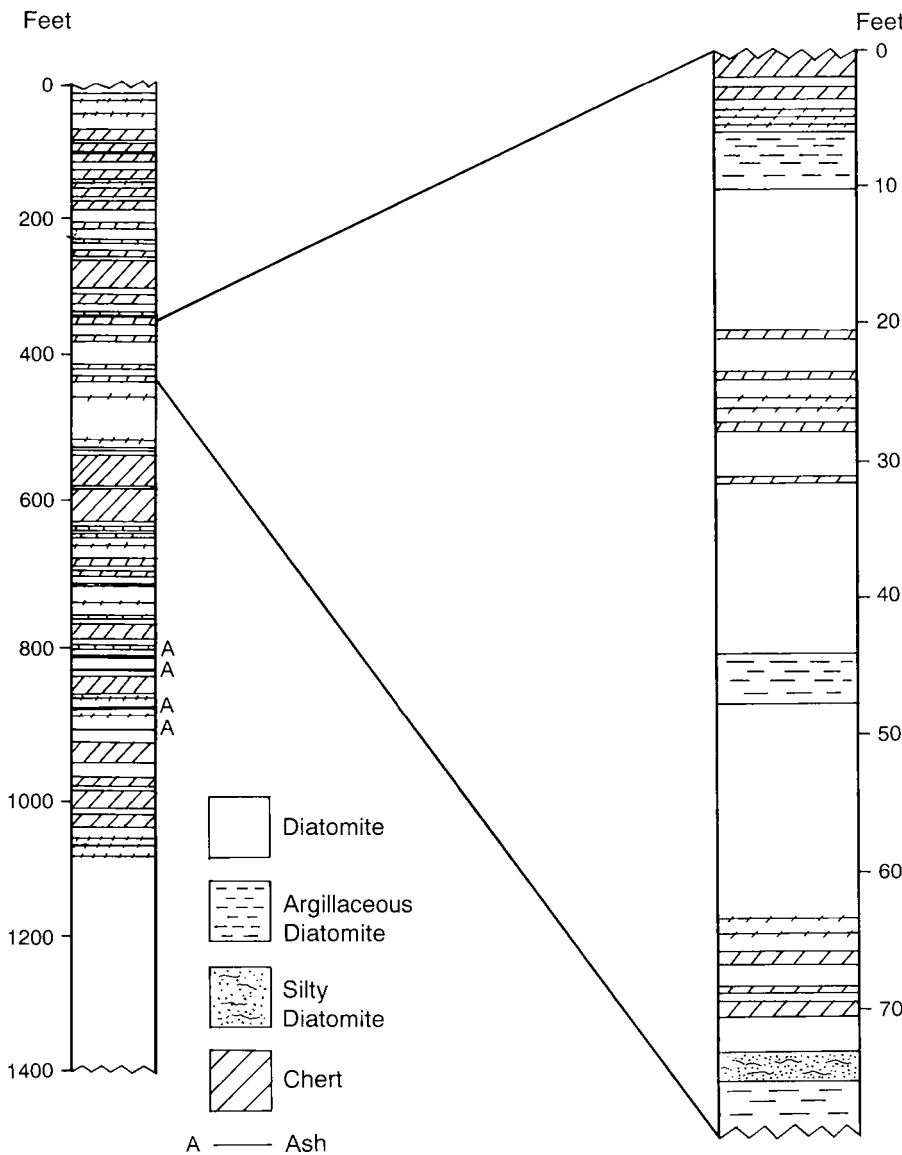
Figure 3. The stratigraphic column of the Monterey Formation sediments in the Lompoc area (left), with an enlargement of the stratigraphy in the Miguelito Mine (right) after Jenkins. 12
