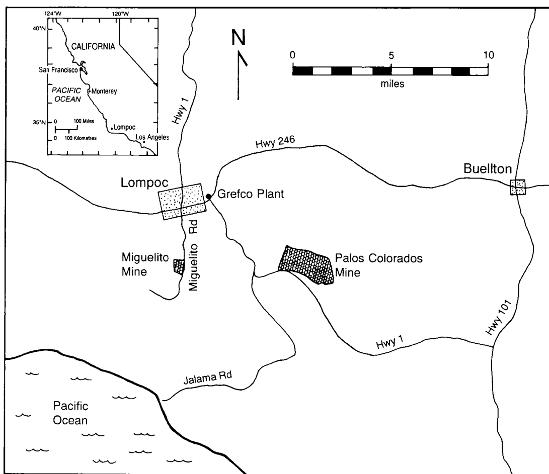
Figure 2. Location map showing the Miguelito Mine near Lompoc in California.
