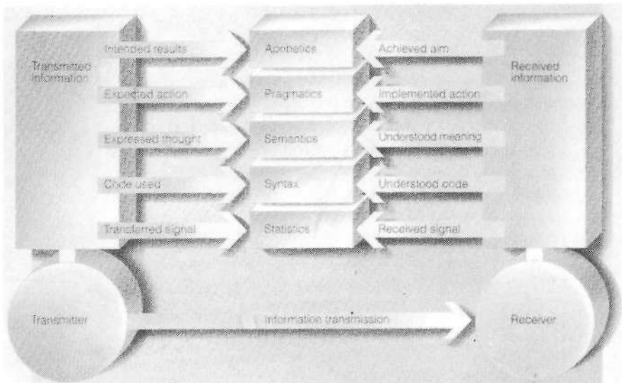
Figure 4. The five mandatory levels of information (middle) begin with statistics (at the lowest level). At the highest level is apobetics (purpose).
