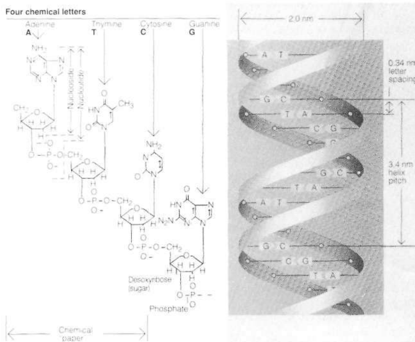
Figure 1. The DNA molecule — the universal storage medium of natural systems. A short section of a strand of the double helix with sugar-phosphate chain reveals its chemical structure (left). The schematic representation of the double helix (right) shows the base pairs coupled by hydrogen bridges (in a plane perpendicular to the helical axis).
