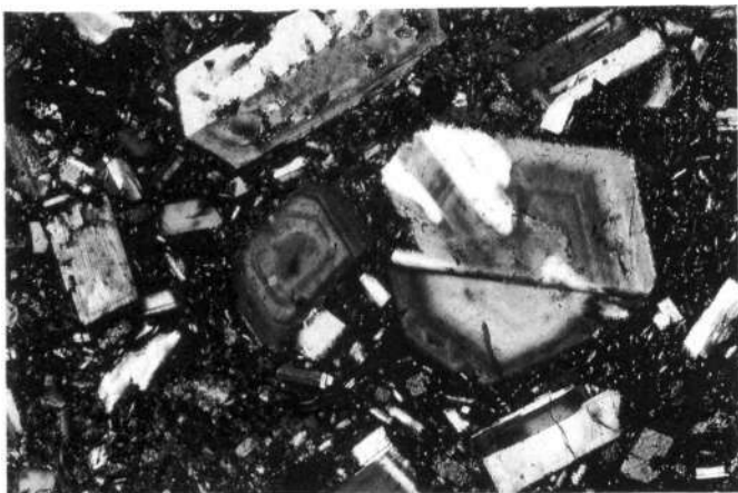
Figure 4. Photomicrograph of Mount St Helens dacite flow of 1986. The most abundant phenocrysts are plagioclase which are embedded in a much finer-grained groundmass containing glass and microphenocrysts. Photographed in polarised light with 2 mm width of view (dacite sample 'DOME-1', photo by A. A. Snelling).
