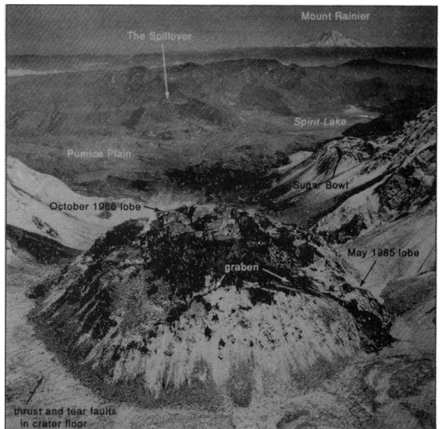
Figure 2. Mount St Helens' new lava dome is composed of 74 million cubic metres of dacite flows and intrusions built up within the crater between October 18, 1980, and October 26, 1986. The view is toward the north looking over the lava dome into the 1980 blast zone (photo by Lyn Topinka of the US Geological Survey, after Pringle, Ret 1).
