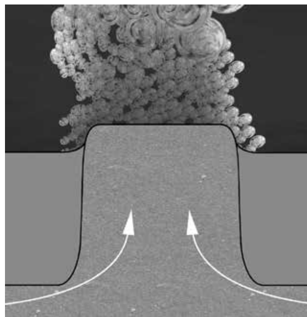
Figure 5. The law of communicating vessels demands equilibrium between the weight of the multiple-kilometres-thick mud layer plus any water above it, and the weight of the salt/steam column within. As the density of steam is relatively low, it favours the rise of the salt pillar. This picture shows the moment the salt protrudes the mud in a sub-oceanic scenario.
